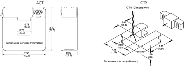
Current Transformer Dimensions
