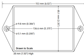
Meter Dimensions
