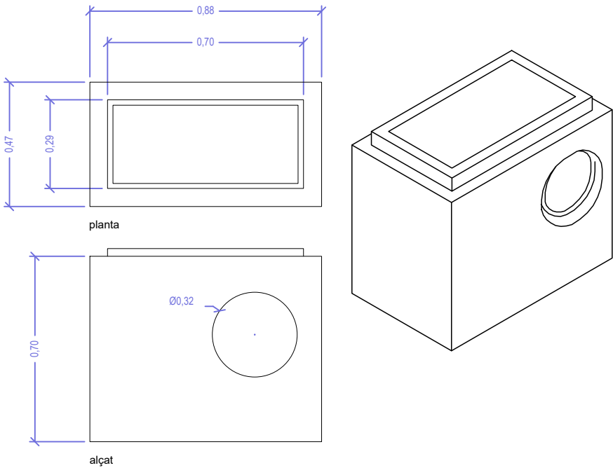
Embornal prefabricat
