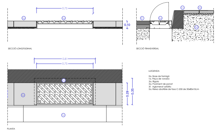
Detall embornal
